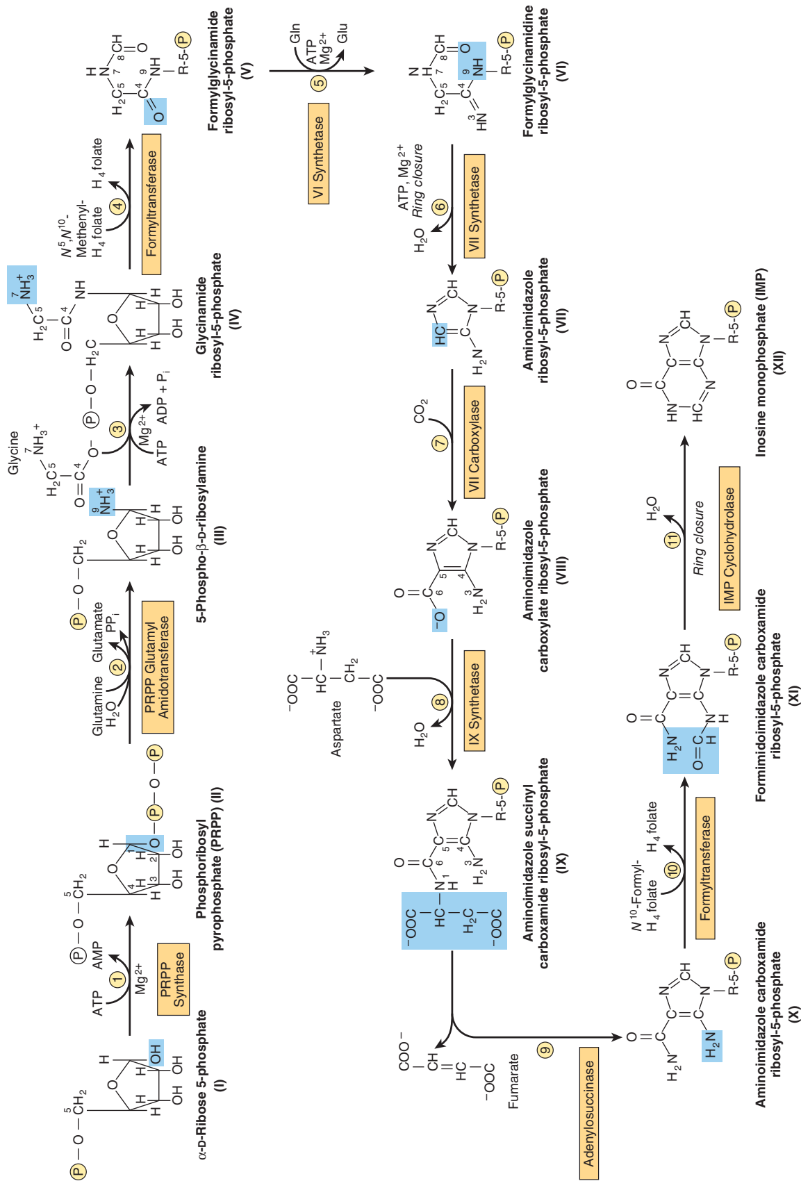
FIGURE 33-2 Purine biosynthesis from ribose 5-phosphate and ATP. See the text for explanations. (P), PO_3^- or PO_2^- .
