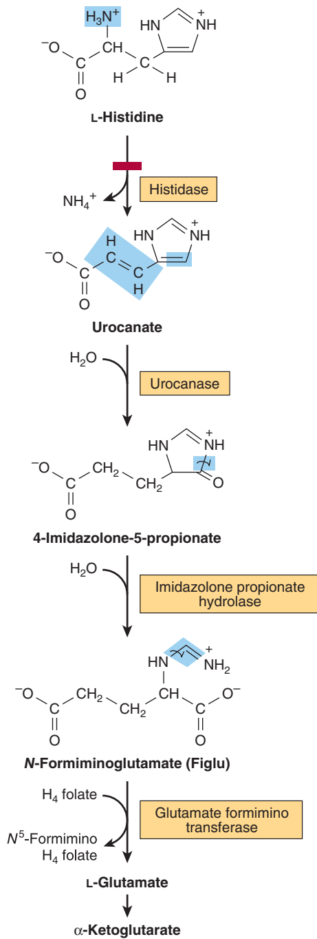
FIGURE 29-5 Catabolism of L-histidine to α-ketoglutarate. ( \text{H}_4 folate, tetrahydrofolate.) The red bar indicates the site of an inherited metabolic defect.
