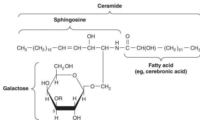
FIGURE 21–15 Structure of galactosylceramide.
