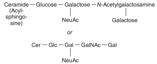
FIGURE 21–16 GM1 ganglioside, a monosialoganglioside, the receptor in human intestine for cholera toxin.
