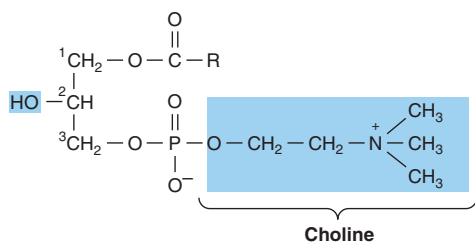
FIGURE 21-13 Lysophosphatidylcholine (lysolecithin).
