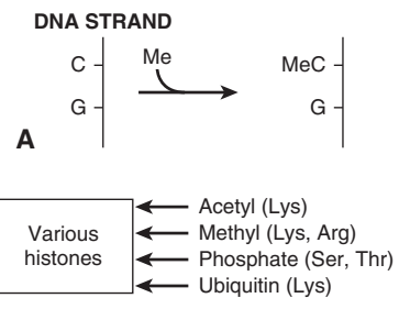
FIGURE 56–13 Some factors involved in epigenetics.
