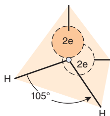
FIGURE 2-1 The water molecule has tetrahedral geometry.
