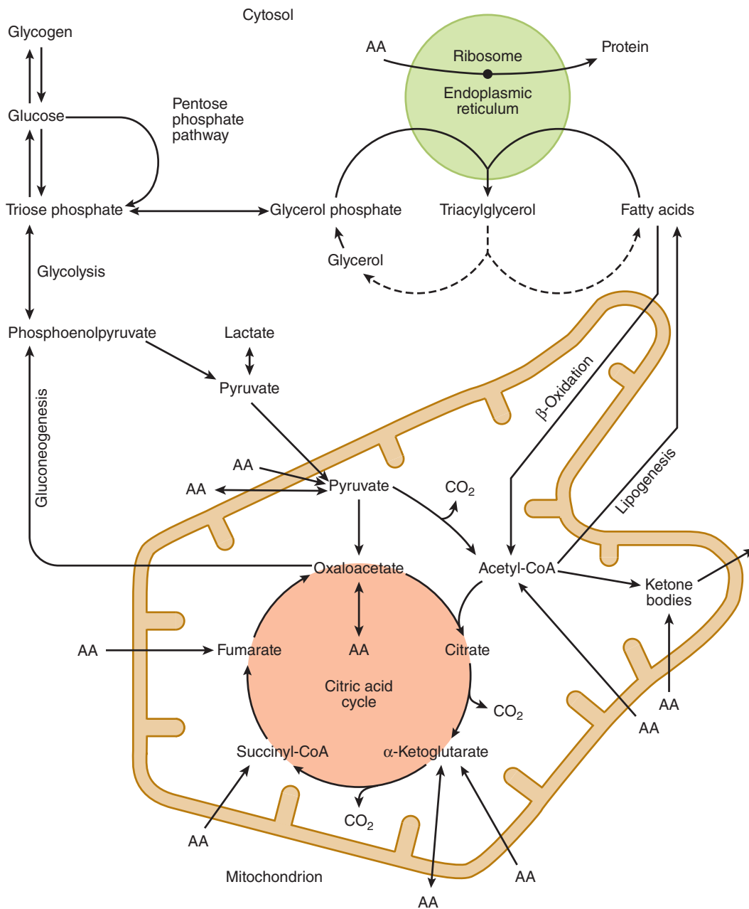
FIGURE 14-7 Intracellular location and overview of major metabolic pathways in a liver parenchymal cell. (AA →, metabolism of one or more essential amino acids; AA ↔, metabolism of one or more nonessential amino acids.)
