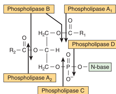
FIGURE 24–6 Sites of the hydrolytic activity of phospholipases on a phospholipid substrate.
