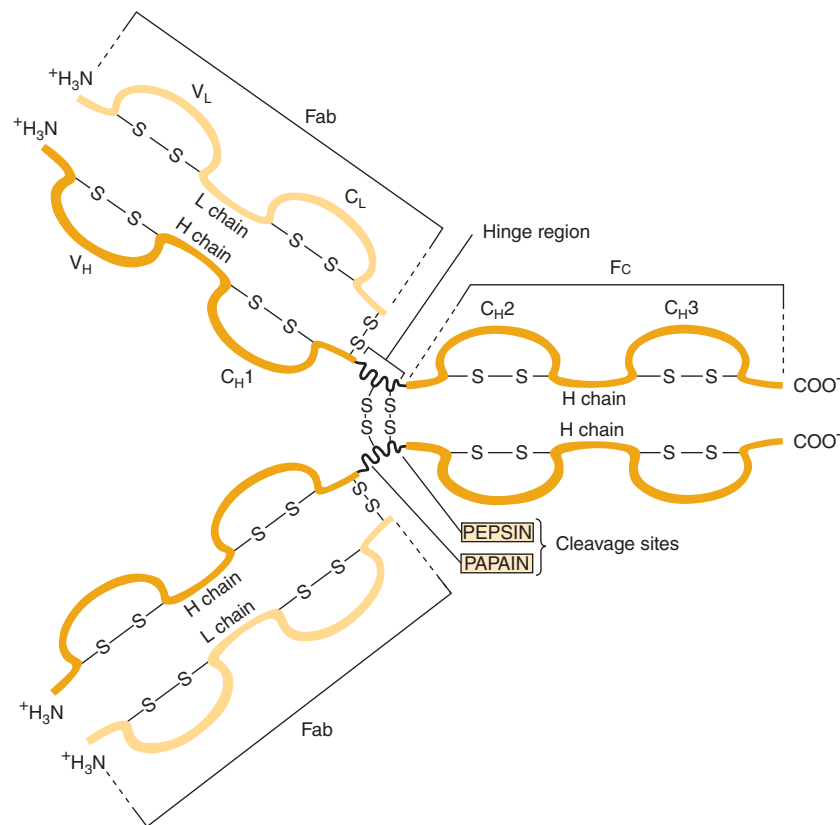
FIGURE 52-11 Structure of IgG. The molecule consists of two light (L) chains and two heavy (H) chains. Each light chain consists of a variable (V L ) and a constant (C L ) region. Each heavy chain consists of a variable region (V H ) and a constant region that is divided into three domains (C H1 , C H2 , and C H3 ). The C H2 domain contains the complement-binding site and the C H3 domain contains a site that attaches to receptors on neutrophils and macrophages. The antigen-binding site is formed by the hypervariable regions of both the light and heavy chains, which are located in the variable regions of these chains (see Figure 50-10). The light and heavy chains are linked by disulfide bonds, and the heavy chains are also linked to each other by disulfide bonds. (Reproduced, with permission, from Parslow TG, et al (editors): Medical Immunology , 10th ed. McGraw-Hill, 2001.)
