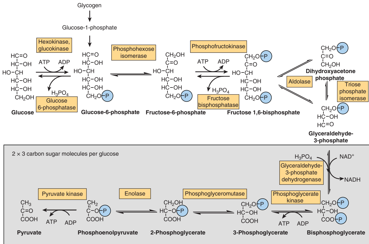
FIGURE 17-2 The pathway of glycolysis. (⊖, — \text{PO}_3^{2-} ; \text{P}_i , \text{HOPO}_3^{2-} ; ⊕, inhibition.) *Carbons 1-3 of fructose bisphosphate form dihydroxyacetone phosphate, and carbons 4-6 form glyceraldehyde-3-phosphate.
