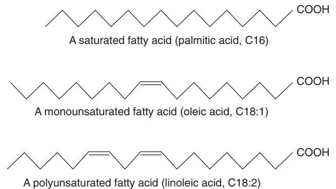
FIGURE 21-1 Fatty acids. Examples of a saturated (palmitic acid), monounsaturated (oleic acid), and a polyunsaturated (linoleic acid) fatty acid are shown.
