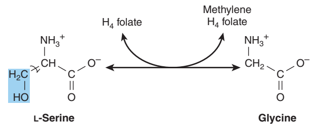
FIGURE 29-7 Interconversion of serine and glycine by glycine hydroxymethyltransferase. ( \text{H}_4 folate, tetrahydrofolate)
