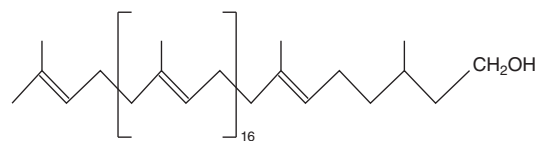
FIGURE 21-23 Dolichol—a C95 alcohol.
