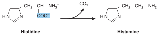
FIGURE 54-1 Structures of histidine and its decarboxylation product, histamine.
