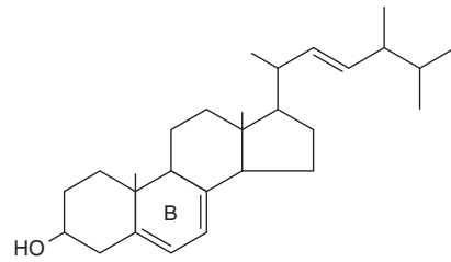
FIGURE 21-21 Ergosterol.
