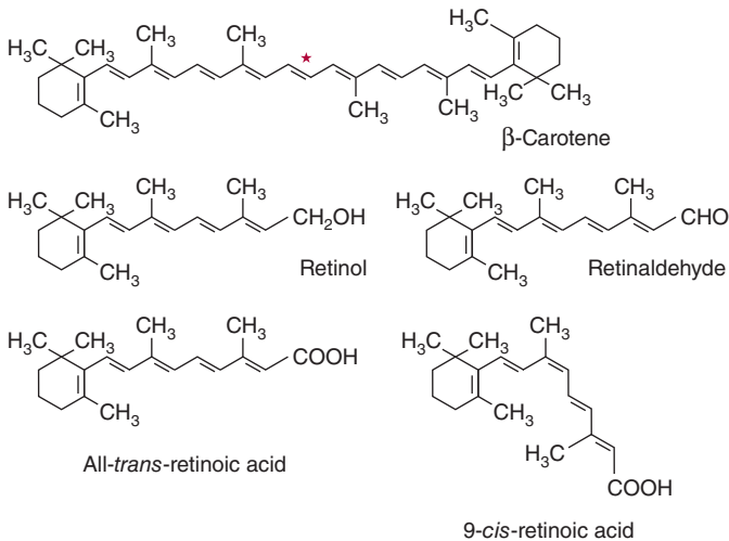
FIGURE 44-1 β-Carotene and the major vitamin A vitamers. Asterisk shows the site of symmetrical cleavage of β-carotene by carotene dioxygenase, to yield retinaldehyde.
