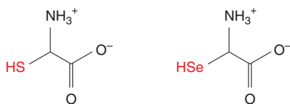
FIGURE 3-1 Cysteine (left) & selenocysteine (right). pK_3 for the selenyl proton of selenocysteine is 5.2. Since this is 3 pH units lower than that of cysteine, selenocysteine represents a better nucleophile at or below pH 7.4.
