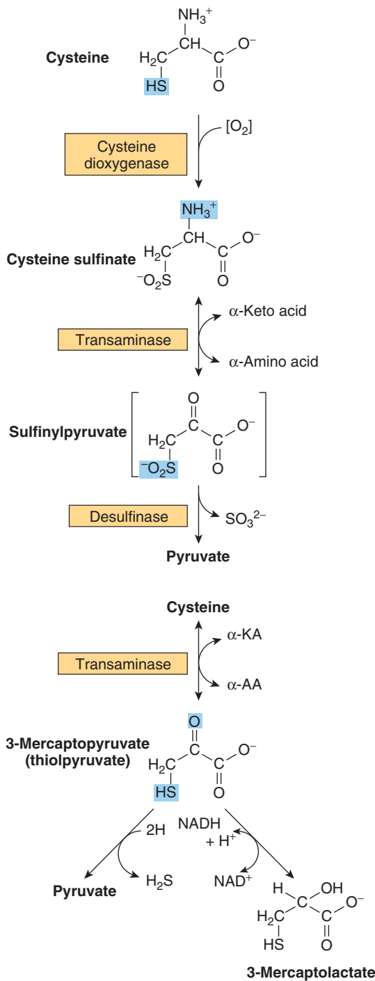
FIGURE 29-9 Two pathways catabolize cysteine: the cysteine sulfinate pathway (top) and the 3-mercaptopyruvate pathway (bottom).
