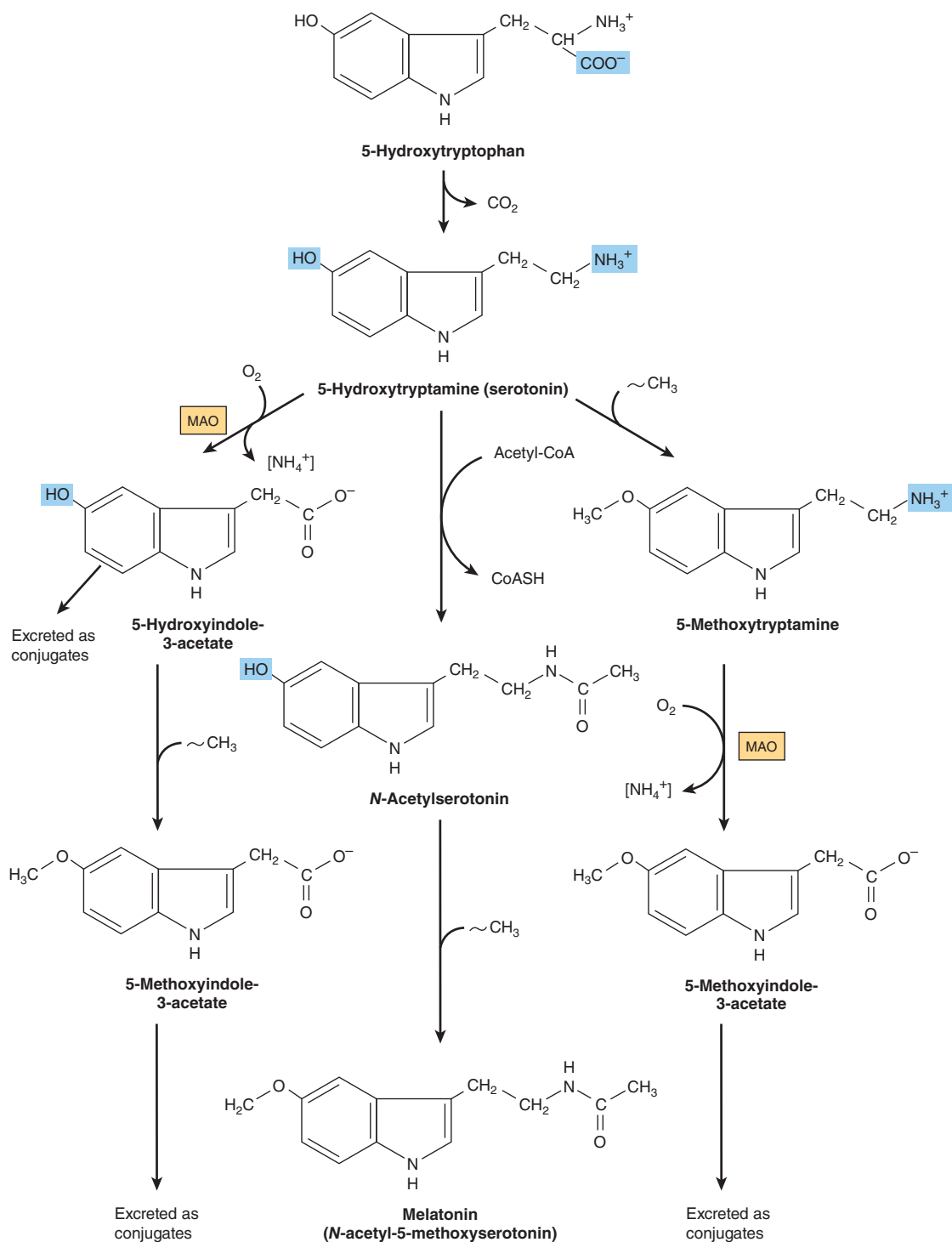
FIGURE 30-11 Biosynthesis and metabolism of serotonin and melatonin. ([NH 4 + ], by transamination; MAO, monoamine oxidase; ~CH 3 , from S-adenosylmethionine.)
