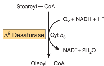
FIGURE 23-9 Microsomal \Delta^9 desaturase.
