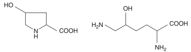
FIGURE 3-2 4-Hydroxyproline & 5-hydroxylysine.
