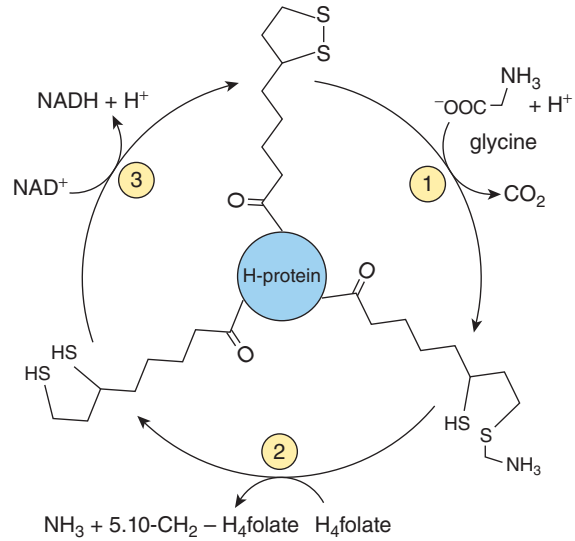
FIGURE 29-6 The glycine cleavage system of liver mitochondria. The glycine cleavage complex consists of three enzymes and an “H-protein” that has covalently attached dihydroliipoate. Catalysts for the numbered reactions are ① glycine dehydrogenase (decarboxylating), ② an ammonia-forming aminomethyltransferase, and ③ dihydroliipoamide dehydrogenase. ( \text{H}_4 folate, tetrahydrofolate).
