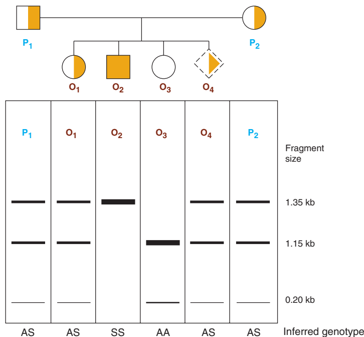
FIGURE 39-9 Pedigree analysis of sickle-cell disease. The top part of the figure (A) shows the first part of the \beta -globin gene and the MstII restriction enzyme sites in the normal (A) and sickle-cell (S) \beta -globin genes. Digestion with the restriction enzyme MstII results in DNA fragments 1.15 kb and 0.2 kb long in normal individuals. The T-to-A change in individuals with sickle-cell disease abolishes one of the three MstII sites around the \beta -globin gene; hence, a single restriction fragment 1.35 kb in length is generated in response to MstII . This size difference is easily detected on a Southern blot. (B) Pedigree analysis shows three possibilities: AA = normal (open circle); AS = heterozygous (half-solid circles, half-solid square); SS = homozygous (solid square). This approach can allow for prenatal diagnosis of sickle-cell disease (dash-sided square). See the text.
