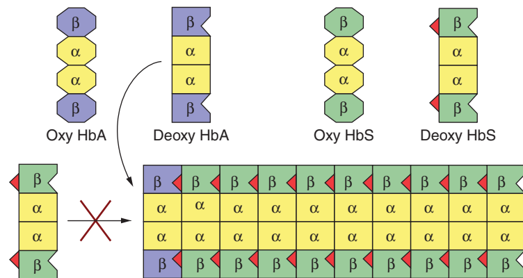
FIGURE 6–13 Polymerization of deoxyhemoglobin S. The dissociation of oxygen from hemoglobin S (HbS) unmasks a sticky patch (red triangle) on the surface of its \beta -subunits (green) that can adhere to a complementary site on the \beta -subunits of other molecules of deoxyHbS. Polymerization to a fibrous polymer is interrupted by deoxyHbA, whose \beta -subunits (lavender) lack the sticky patch required for binding additional HbS subunits. (Modified and reproduced, with permission, from Stryer L: Biochemistry , 4th ed. Freeman, 1995. Copyright © 1995 W. H. Freeman and Company.)
