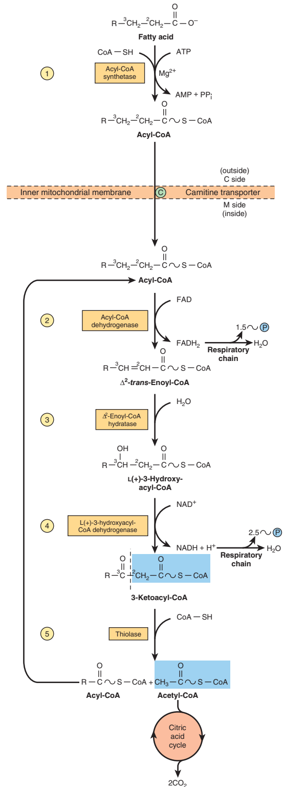
FIGURE 22–3 \beta -Oxidation of fatty acids. Long-chain acyl-CoA is cycled through reactions 2–5, acetyl-CoA being split off, each cycle, by thiolase (reaction 5). When the acyl radical is only four carbon atoms in length, two acetyl-CoA molecules are formed in reaction 5.
