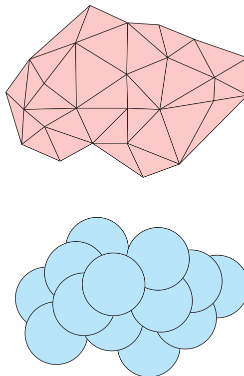
FIGURE 10-6 Simplified digital representations of the surface topography of a molecule using either triangular panels or an assembly of spheres.
