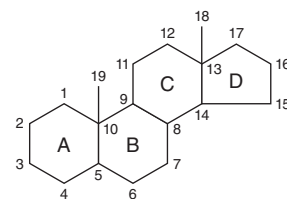
FIGURE 21–17 The steroid nucleus.
