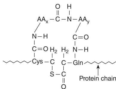
FIGURE 52–10 An internal cyclic thiol ester bond, as present in \alpha_2 -macroglobulin. AA x and AA y are neighboring amino acids to cysteine and glutamine.
