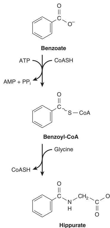
FIGURE 30-5 Biosynthesis of hippurate. Analogous reactions occur with many acidic drugs and catabolites.
